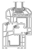
IDEAL 5000® (presek)
